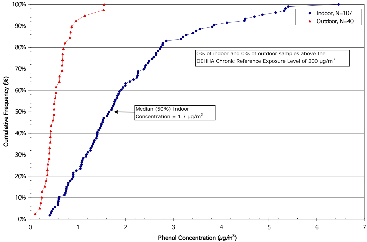
Figure 18. Phenol concentration cumulative frequency distribution – All Home Sample Frame.
