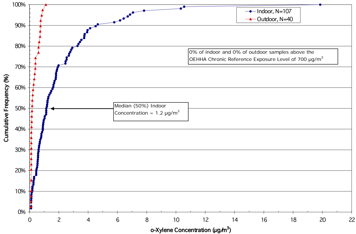
Figure 25. o-Xylene concentration cumulative frequency distribution – All Home Sample Frame.
