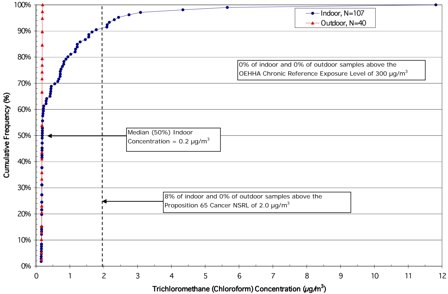
Figure 22. Trichloromethane (chloroform) cumulative frequency distribution – All Home Sample Frame.
