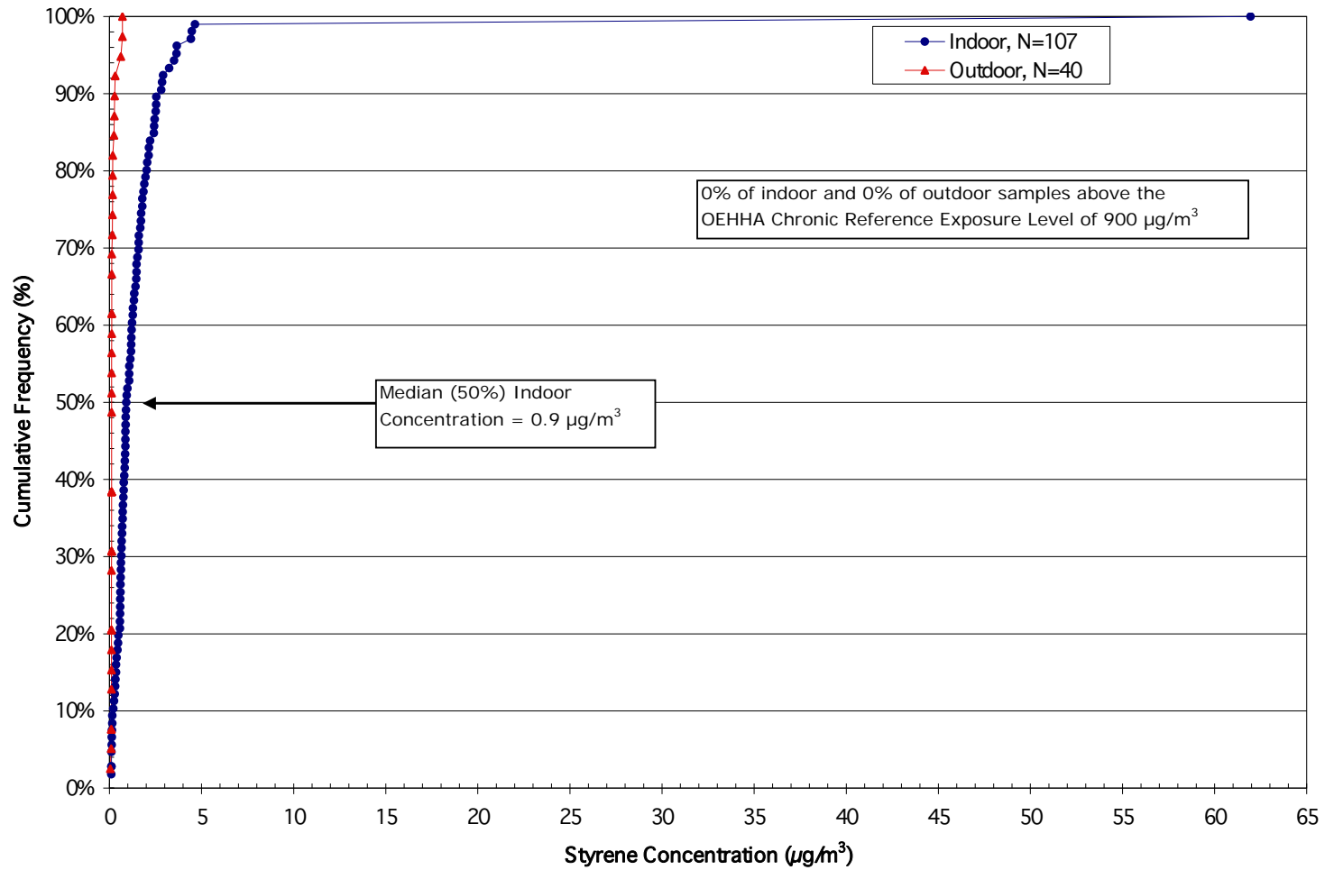
Figure 19. Styrene concentration cumulative frequency distribution – All Home Sample Frame.
