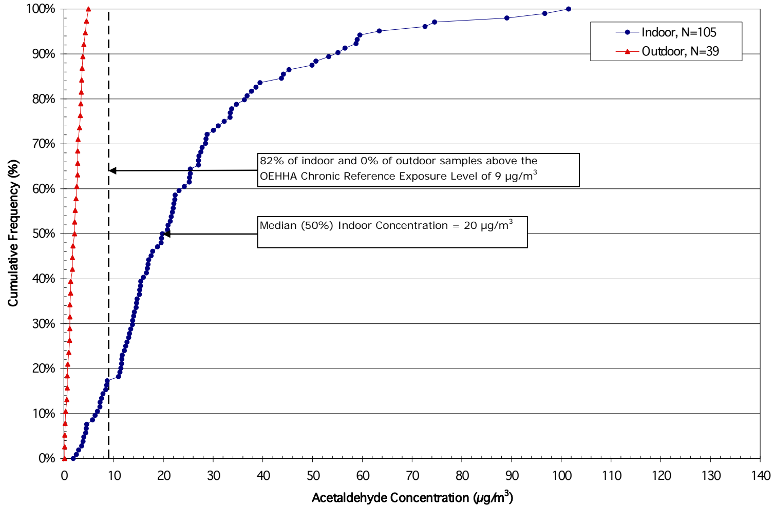
Figure 27. Acetaldehyde concentration frequency distribution – All Home Sample Frame.
