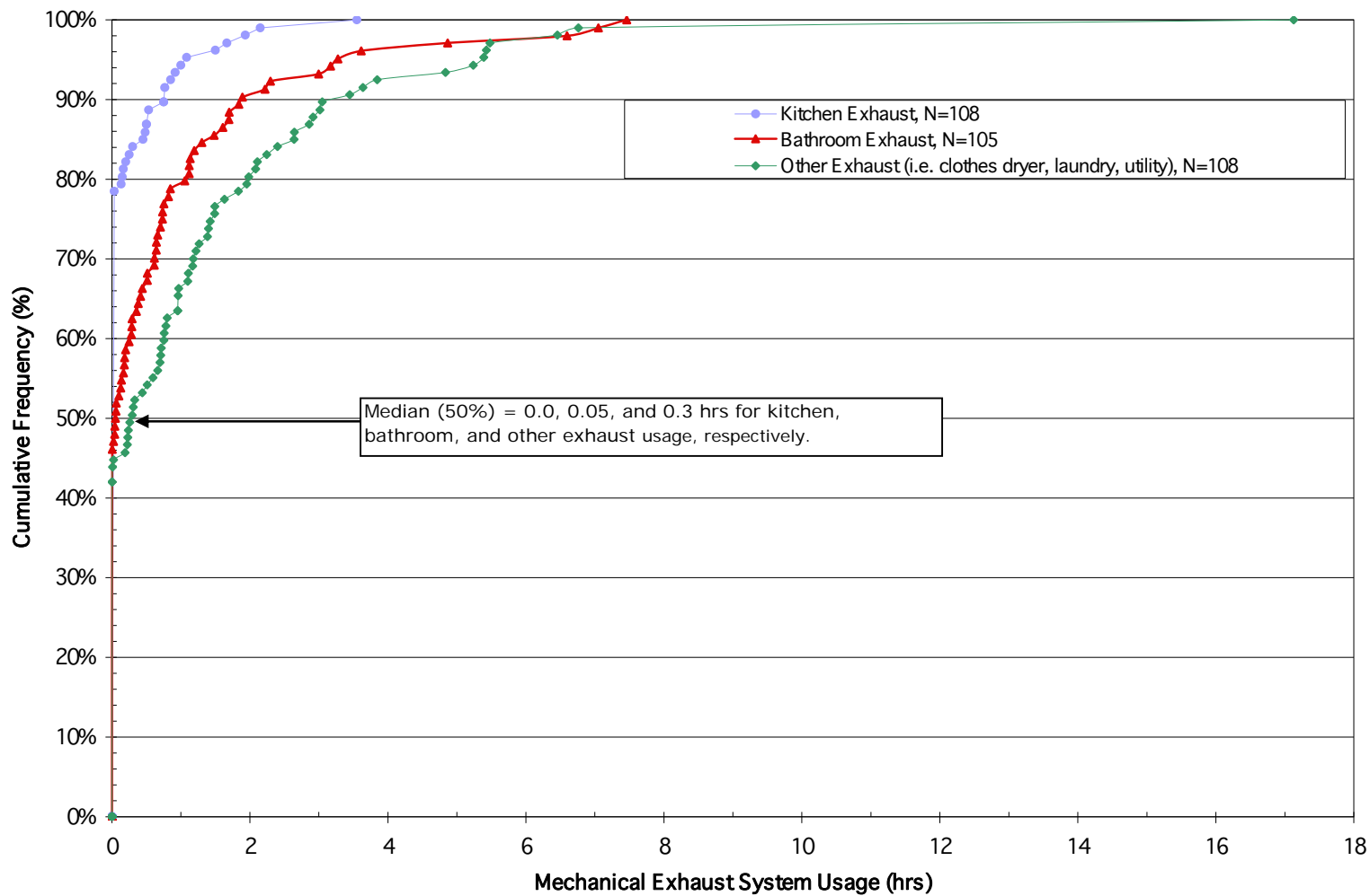
Figure 7. Mechanical exhaust system usage cumulative frequency distribution – All Home Sample Frame.
