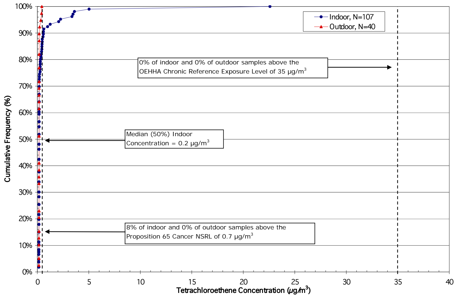
Figure 20. Tetrachloroethene concentration cumulative frequency distribution – All Home Sample Frame.
