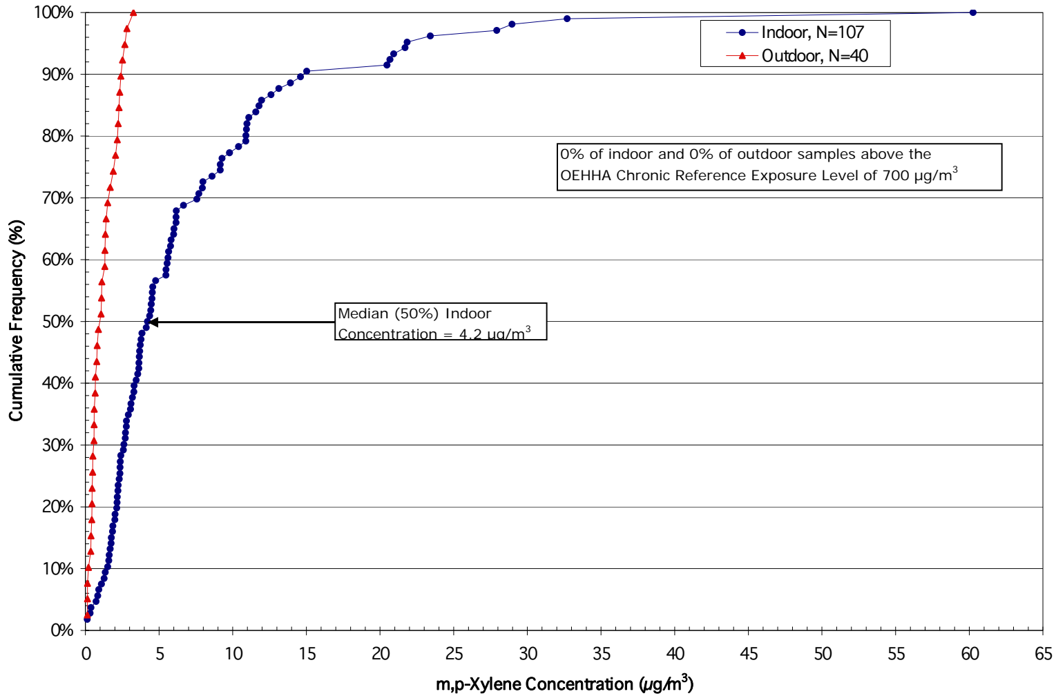
Figure 24. m,p-Xylene concentration cumulative frequency distribution – All Home Sample Frame.
