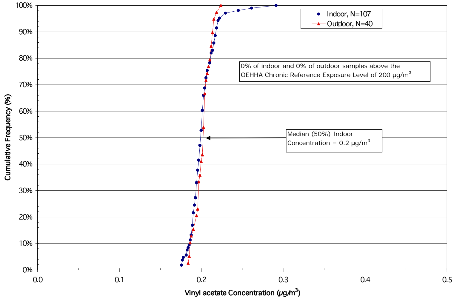
Figure 23. Vinyl acetate concentration cumulative frequency distribution – All Home Sample Frame.
