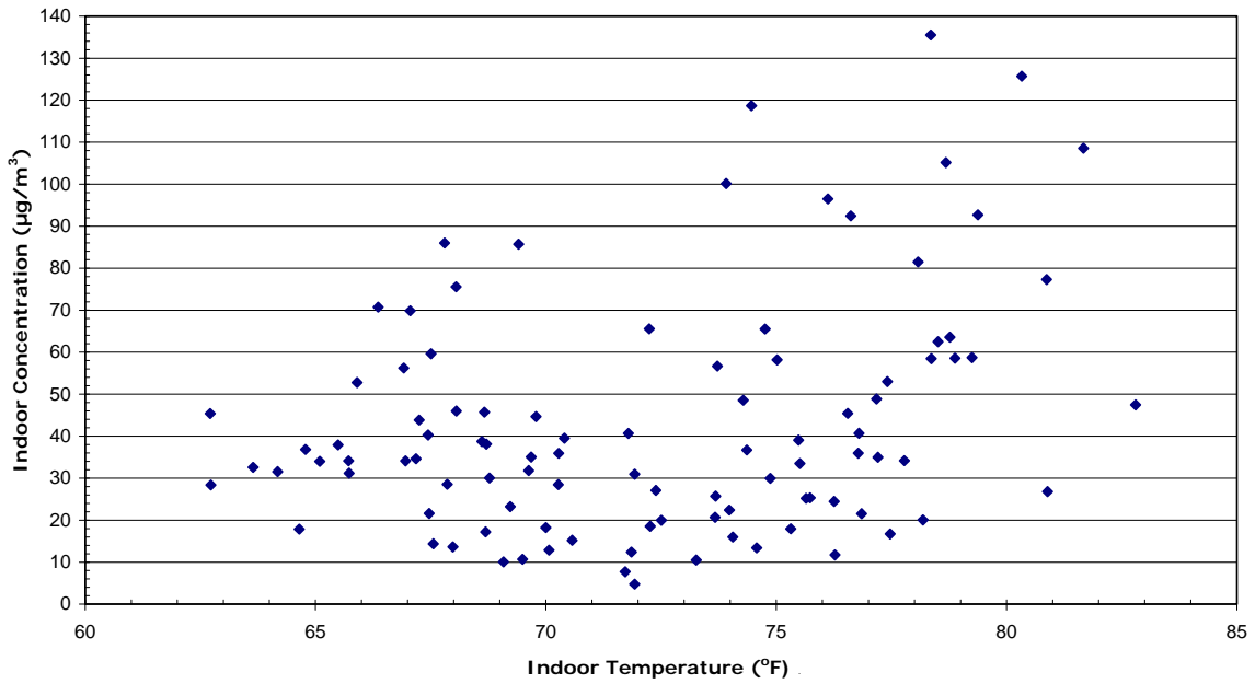
Scatter Plot of Indoor Temperature and Indoor Acetaldehyde Concentrations All Homes Sample Frame
