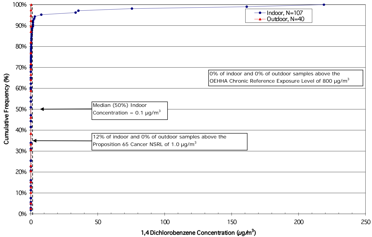
Figure 14. 1,4 Dichlorobenzene concentration cumulative frequency distribution –All Home Sample Frame.
