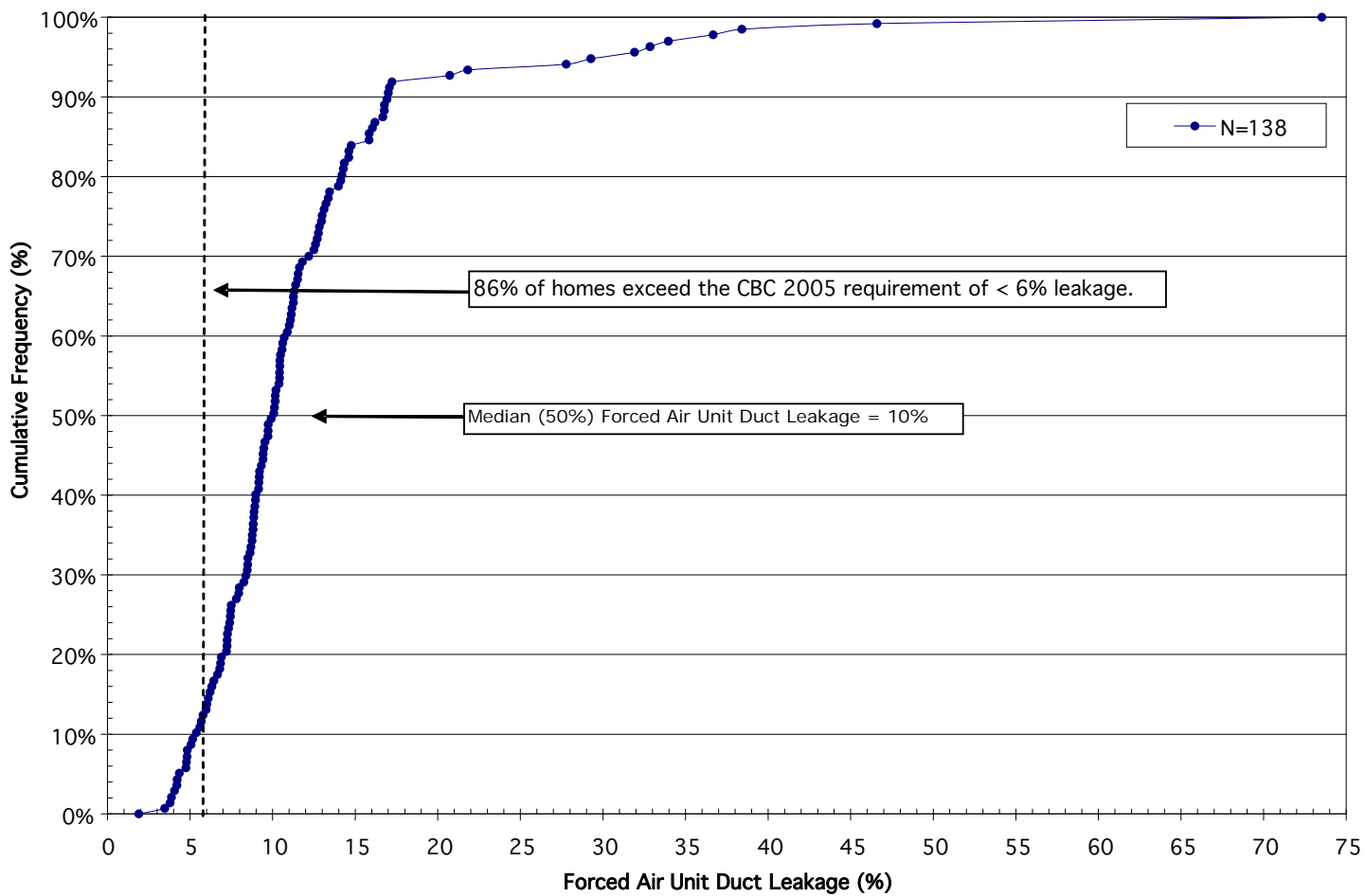
Figure 4. Forced air duct leakage cumulative frequency distribution - All Home Sample Frame.
