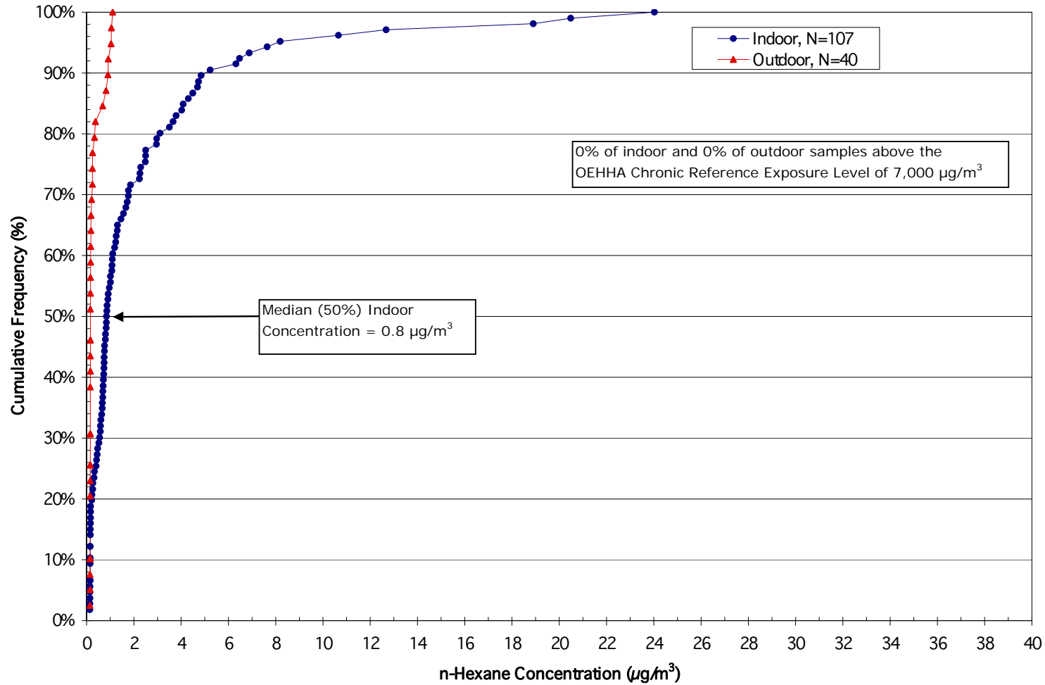
Figure 16. n-Hexane concentration cumulative frequency distribution – All Home Sample Frame.
