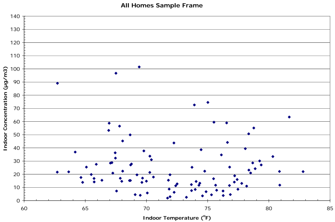
Scatter Plot of Indoor Temperature and Indoor Acetaldehyde Concentrations All Homes Sample Frame
